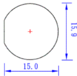
Mounting Holes
