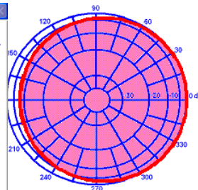
VERTICAL RADIATION PATTERN
