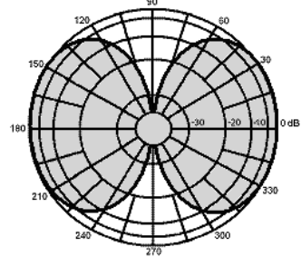
HORIZONTAL RADIATION PATTERN
