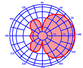
HORIZONTAL RADIATION PATTERN
