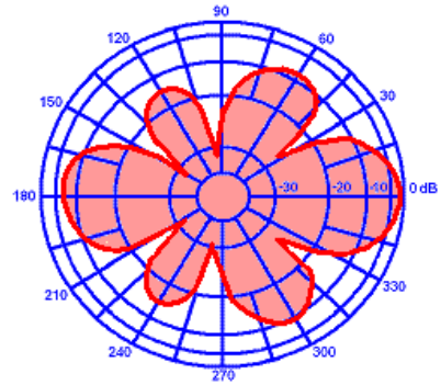
HORIZONTAL RADIATION PATTERN
