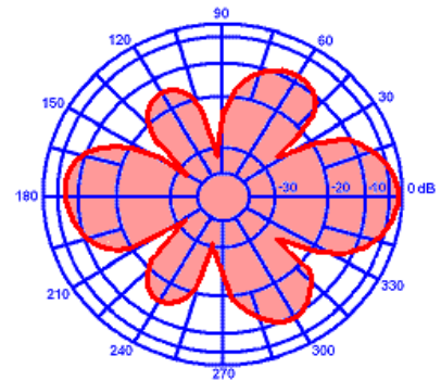
HORIZONTAL RADIATION PATTERN
